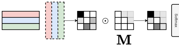
Figure E.11.1: Visual depiction of causal attention implemented with attention masking.
