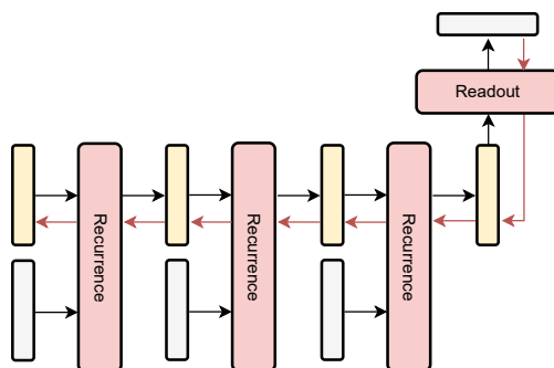
Figure E.13.2: Backward pass for a recurrent layer: the adjoint values have to be propagated through all the transition steps. Each state then contributes a single term to the full gradient of the parameters.
