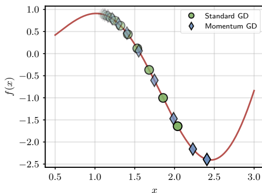
Figure F.2.4: GD and GD with momentum when minimizing the function x \sin(2x) starting from x = 1 + \varepsilon , with \lambda = 0.3 .
