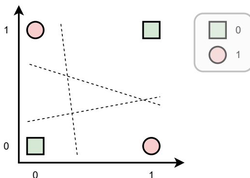
Figure E.5.1: Illustration of the XOR dataset: green squares are values of one class, red circles are values of another class. No linear model can separate them perfectly (putting all squares on one side and all circles on the other side of the decision boundary). We say that the dataset is not linearly separable .
