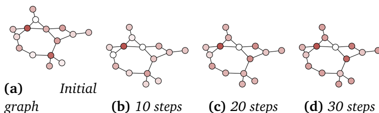
Figure E.12.4: (a) A random graph with 15 nodes and a scalar feature on each node (denoted with variable colors). (b)-(d) The result after 10, 20, and 30 steps of diffusion with the Laplacian matrix. The features converge to a stable state.
