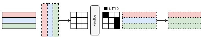
Figure E.10.3: SA with a “hard” attention is equivalent to a vector-valued dictionary.
