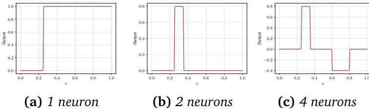
Figure F.B.2: (a) A neural network with one input, one hidden neuron, and one output can approximate any step function (here shown with a = 1 and s = 0.3 ). (b) With two hidden neurons and one output we can approximate any function which is constant over a small interval. (c) With four neurons, we can approximate any function which is piecewise constant over two non-zero intervals. Note that bins can be negative by defining a negative amplitude.
