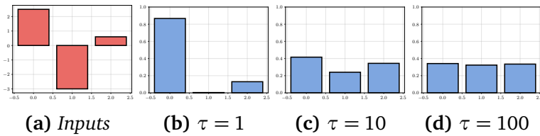
Figure E.4.3: Example of softmax applied to a three-dimensional vector (a), with temperature set to 1 (b), 10 (c), and 100 (d). As the temperature increases, the output converges to a uniform distribution. Note that inputs can be both positive or negative, but the outputs of the softmax are always constrained in [0, 1] .
