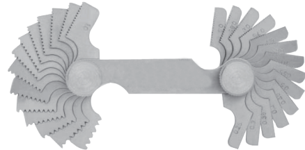
Thread Pitch Gauge
