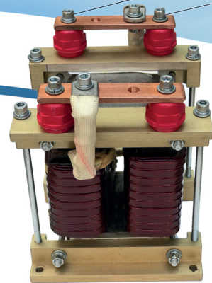
200A-400HZ
