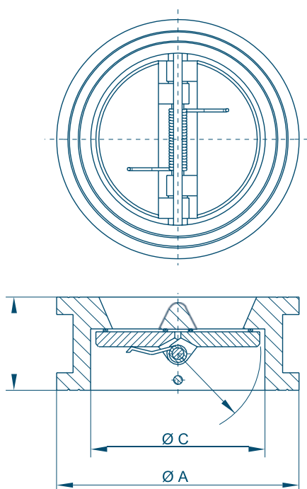
Double check valve
